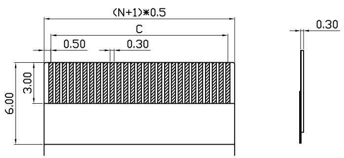
RECOMMENDED FFC/FPC DIM.
